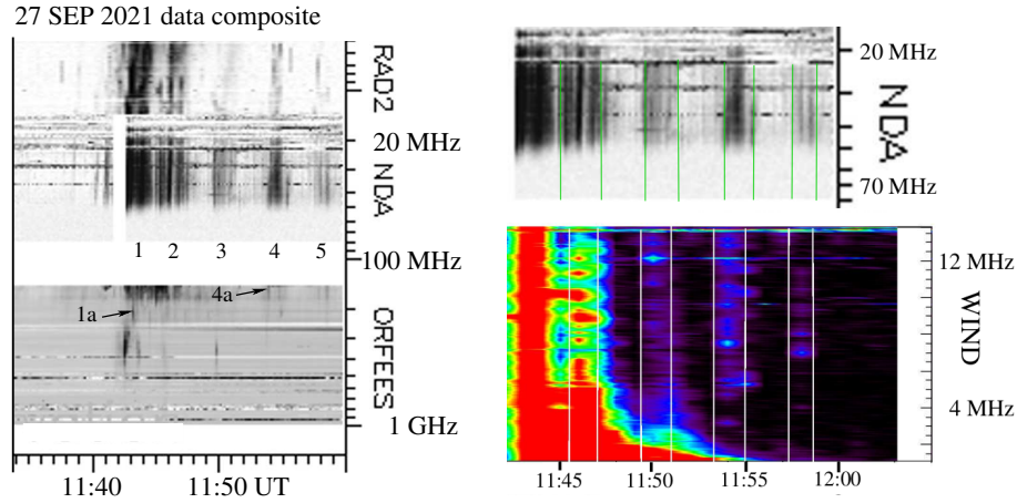
Figure 4. Radio monitoring composite showing observed radio emission in the dynamic spectra for the 27 September 2021 event. Numbers 1–5 refer to the type III burst groups. The locations of bursts labelled 1a and 4a are shown in Figures 7 and 6, respectively. Comparison between NDA and Wind /WAVES spectra is also shown.
