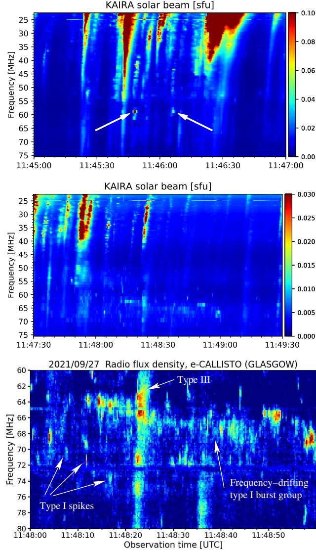
Figure 8. Dynamic spectrum taken during the second group of type III bursts show narrow-band enhanced plasma emission features, these are indicated with arrows in the KAIRA observations at 75–25 MHz ( top ). Narrow-band spikes (type I noise storm features) were observed in between the type III burst groups (KAIRA observations, middle ). e-CALLISTO GLASGOW dynamic spectrum at 80–60 MHz shows the spikes and spike burst groups in more detail ( bottom ).
