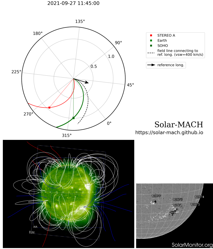
Figure 2. Top: Spacecraft locations on 27 September 2021. The STEREO-A spacecraft longitude separation to Earth was 39.8 degrees, with SOHO, SDO, Wind , and Fermi spacecrafts at Earth’s longitude. The reference longitude is for the B4.5-class flare located at S29W35. (Plot prepared with Solar-MACH, The Solar Magnetic Connection HAUS tool.) Bottom left: STEREO-A/EUVI image rotated to SDO/AIA field of view, with PFSS magnetic field lines. Blue and red lines indicate open field with opposite polarities and white lines indicate closed field. Bottom right: SDO/HMI magnetogram of the eruption region (from SolarMonitor.org ).
