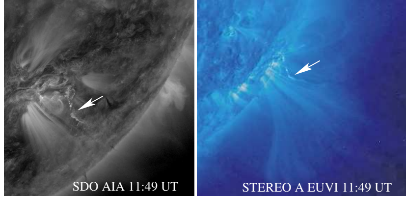
Figure 3. SDO/AIA and STEREO-A/EUVI images of the AR and its surroundings at 11:49 UT. Arrow points to the ejected filament/plasmoid structure. Note the bending of the structure along the magnetic field lines.
