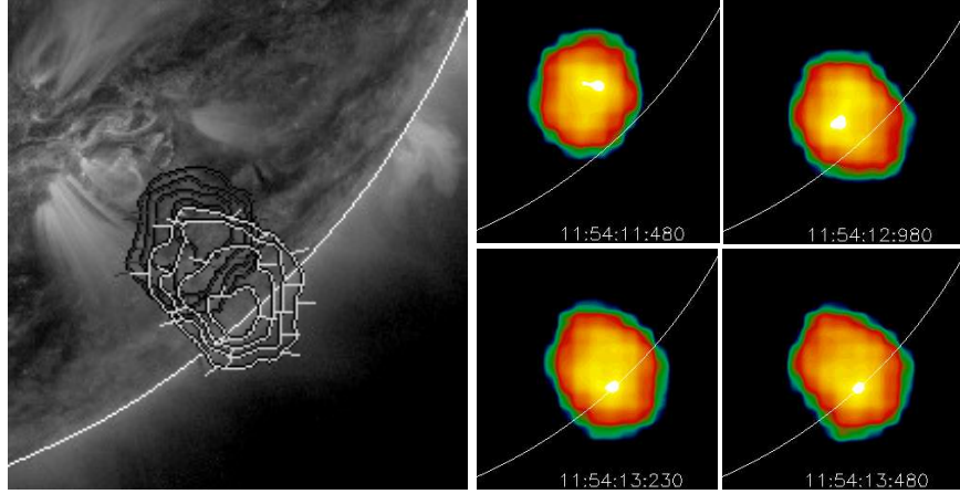
Figure 6. Temporal evolution of burst locations at 150 MHz, observed with NRH. The sources are shown near burst start ( black contours ) and burst end ( white contours ), overplotted on an EUV image ( left ). The spatial evolution is also shown in the color images, from 11:54:11 to 11:54:13 UT ( right ). This spectral feature is marked 4a (within group 4 bursts) in Figure 4. The radio source locations are typical for all type III bursts in the type III burst groups observed at 150 MHz.
