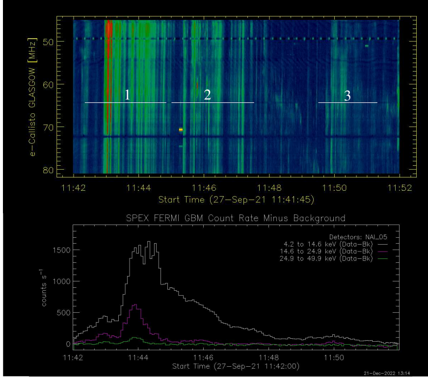
Figure 5. Fermi /GBM background-subtracted X-ray counts from the most sunward-pointing detector at 11:42–11:52 UT ( bottom ). The energy ranges are 4–15 keV, 15–25 keV, and 25–50 keV. Radio dynamic spectrum from e-CALLISTO Glasgow is shown on top , at frequency range 45–81 MHz. Numbers and lines indicate the type III burst groups and their durations.
