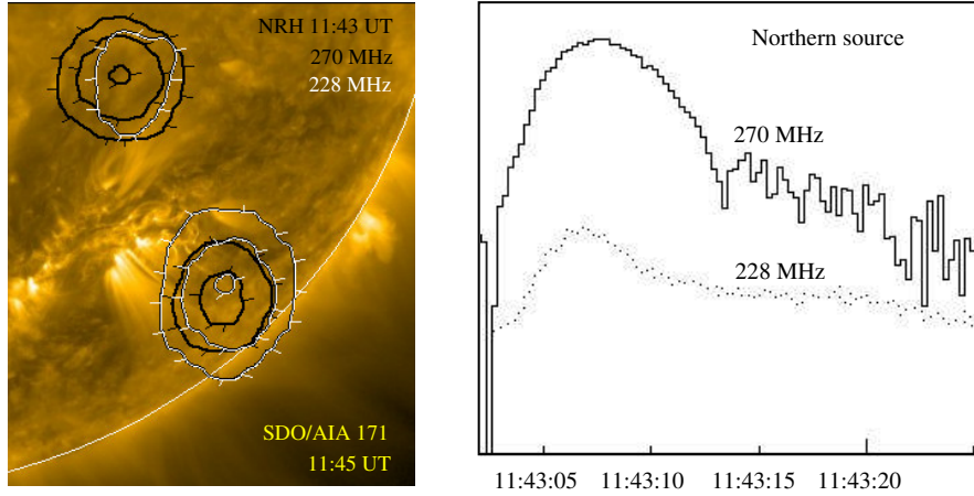
Figure 7. NRH source contours at 270 MHz ( black ) and 228 MHz ( white ) at 11:43:08 UT, plotted over an EUV image ( left ). The spectral feature is marked 1a within group 1 bursts) in Figure 4. The flux curves ( on the right ) of the northern region show an enhancement at 270 MHz, which peaks later than the emission at 228 MHz. This suggests that the electron beam was moving down in the solar atmosphere. The later type III burst groups did not show this northern region again.
