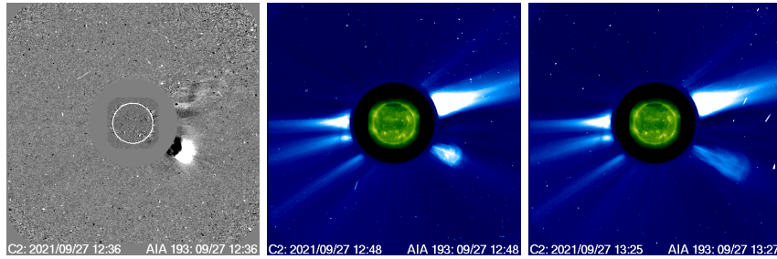
Figure 11. SDO/AIA 193 Å and SOHO/LASCO-C2 difference image at 12:36 UT ( left ), and direct AIA and C2 images at 12:48 UT ( middle ) and 13:25 UT ( right ). The CME was very compact and had a narrow width. No streamers were visible along the CME propagation path.
