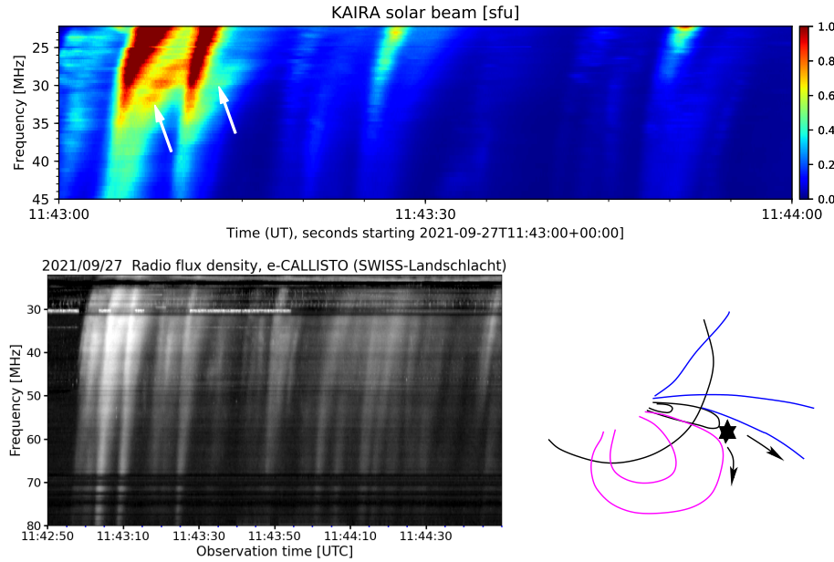
Figure 9. KAIRA observations of V-shaped type III bursts at 11:43 UT ( top ). Arrows point to the change in emission lane direction, visible at 35–27 MHz. The bursts were also observed by several e-Callisto stations, the dynamic spectrum shown here is from the SWISS-Landschlacht e-CALLISTO at 80–20 MHz ( bottom left ). Cartoon shows a possible configuration for the creation of V-shaped type III bursts. Star indicates reconnection and arrows show the directions of two particle beam paths, one along open field lines (emission with constantly decreasing frequencies) and the other following closed loops back to the Sun (emission lane turning back towards lower frequencies).
