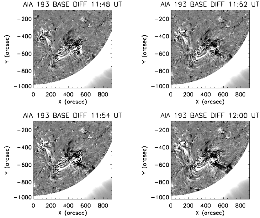
Figure 10. SDO/AIA 193 Å base difference images (base at 11:32 UT). The narrow-width dimming region, located from the AR towards the south-west limb, matches with the type III burst regions imaged at 150 MHz, and also with the CME propagation direction.
