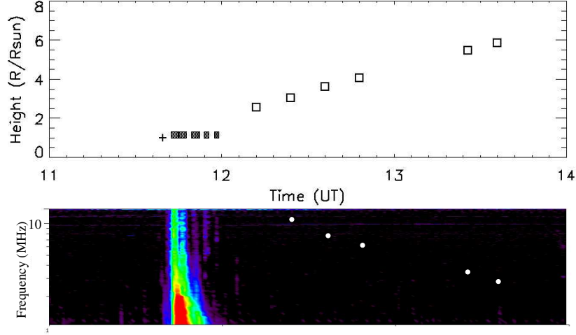
Figure 12. Top: CME leading front heights ( boxes ), the heights are from the LASCO CME Catalog, flare start time ( cross ), and metric type III burst group durations ( filled boxes ). Bottom: Wind/WAVES dynamic spectrum where white circles mark the CME leading front heights converted to frequencies with the hybrid atmospheric density model.
